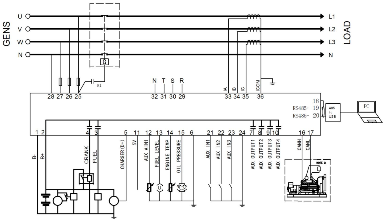
EFI Typical Application
